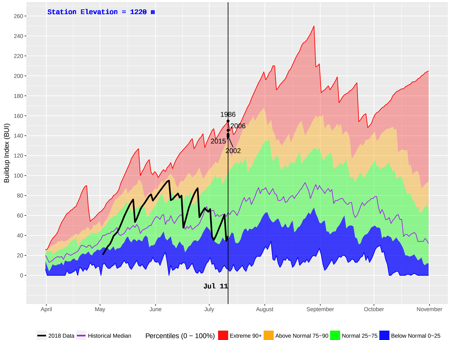
NEMIAH (216) : Historical (1982–2016) and Current (2018) Noon Buildup Index (BUI)
