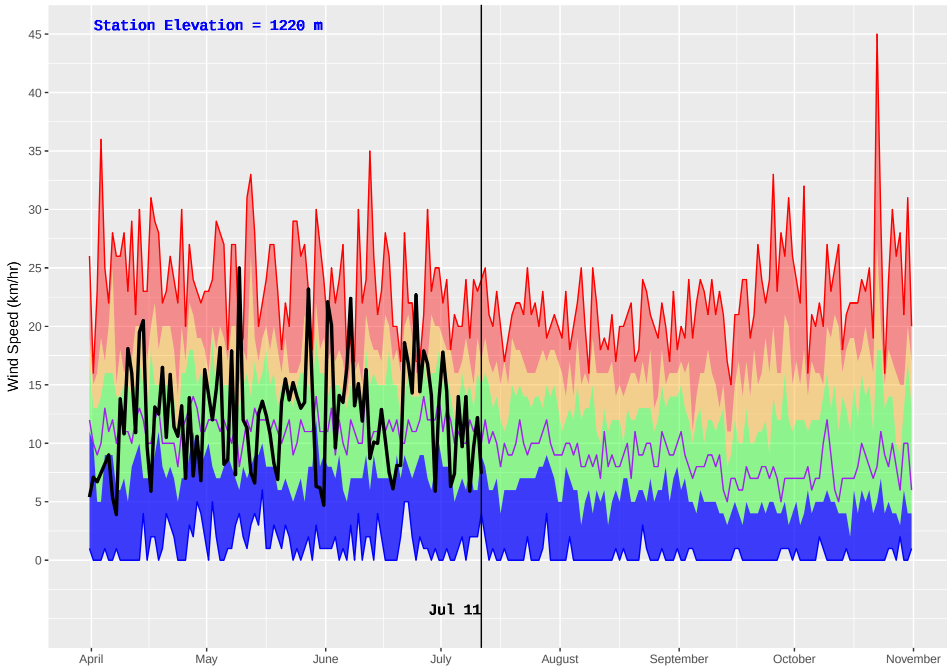
NEMIAH (216) : Historical (1982–2016) and Current (2018) Noon Wind Speed
