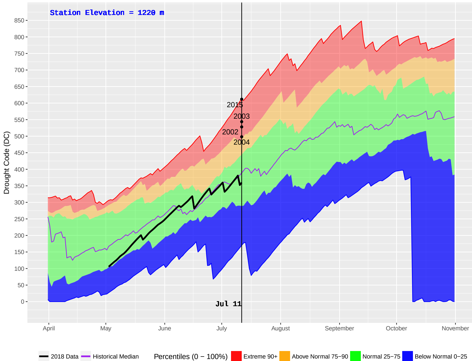
NEMIAH (216) : Historical (1982–2016) and Current (2018) Noon Drought Code (DC)
